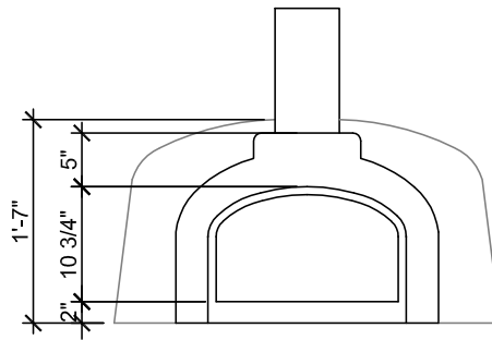
02 FRONT ELEVATION
