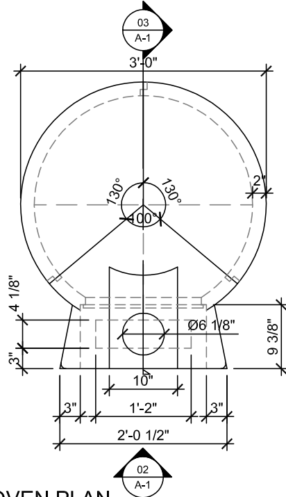
01 OVEN PLAN
